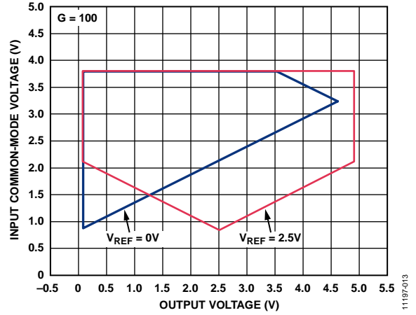
Figure 13. Input Common-Mode Voltage vs. Output Voltage ( G = 100 ), Single-Supply, V_S = 5\text{ V}
