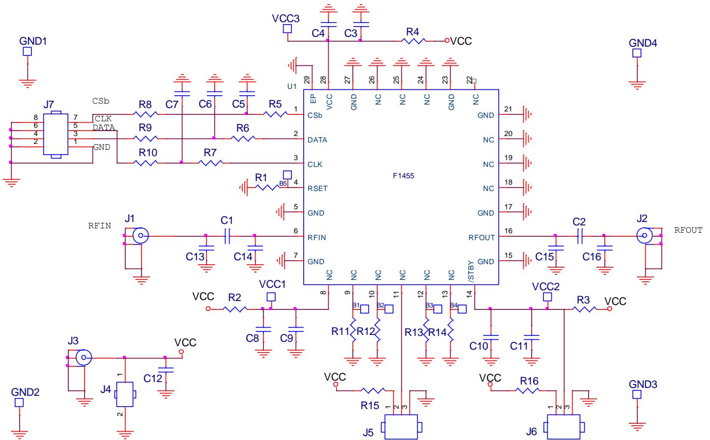
Figure 55. Electrical Schematic
