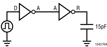
Figure 5. V.10/V.28 Receiver Test Circuit
