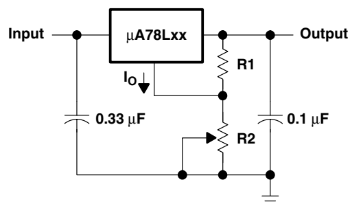
Figure 3. Adjustable-Output Regulator
