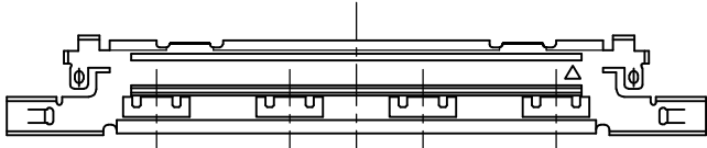
AS SHOWN : 5-2023347-3(40P)
