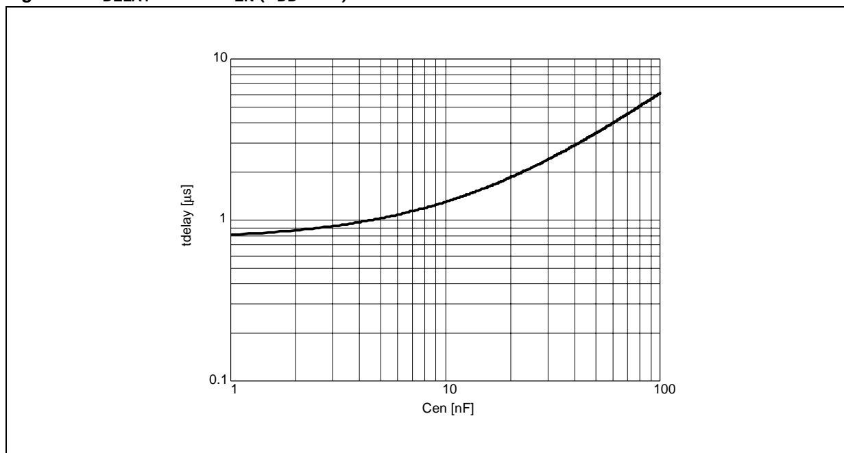
Figure 15. t_{\text{DELAY}} versus C_{\text{EN}} ( V_{\text{DD}} = 5\text{V} ).
