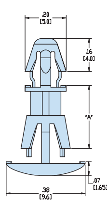
ARROWHEAD SNAP LOCK / REVERSE BUTTON LOCK
