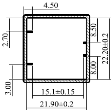
Profile view
