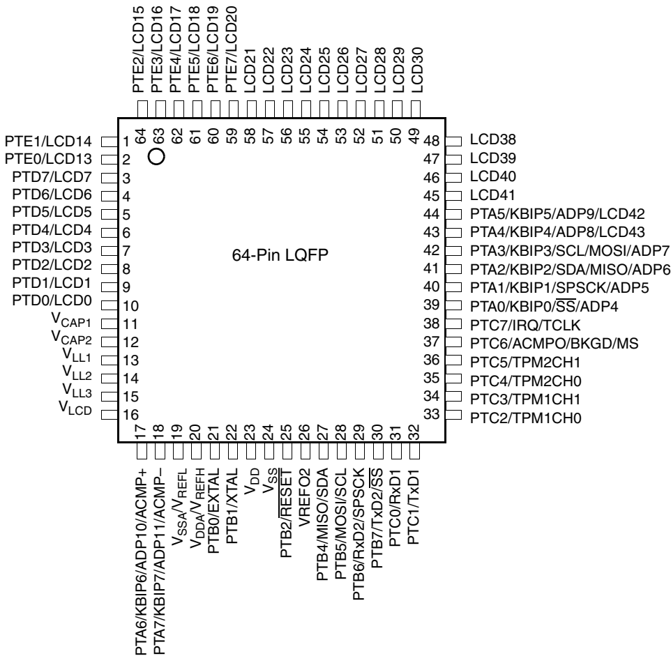
Figure 2. 64-Pin LQFP
