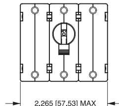
3-POLE (BB3)
