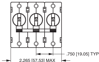
3-POLE (BA3)
