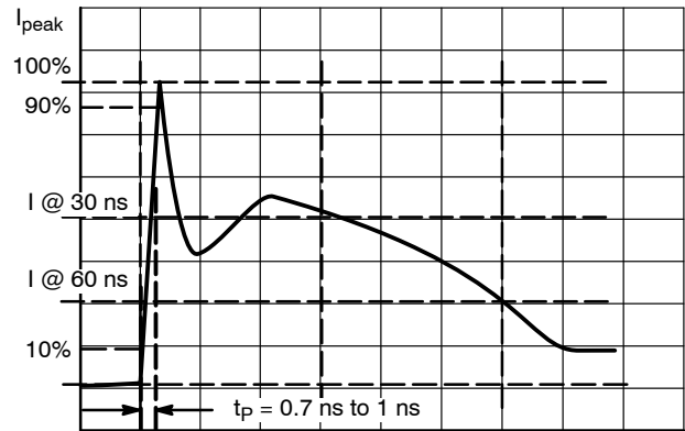
IEC61000-4-2 Waveform
