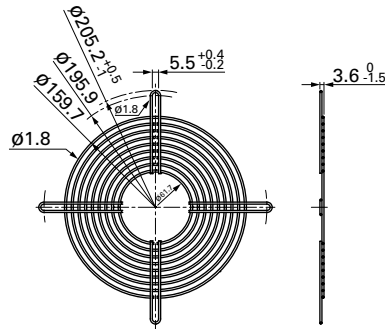
Outlet side
