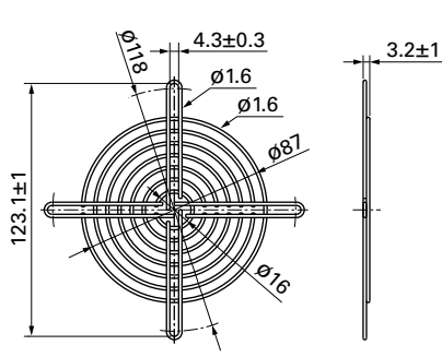
Inlet side
