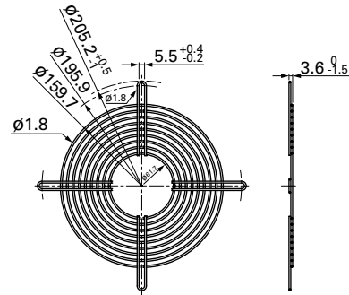
Outlet side
