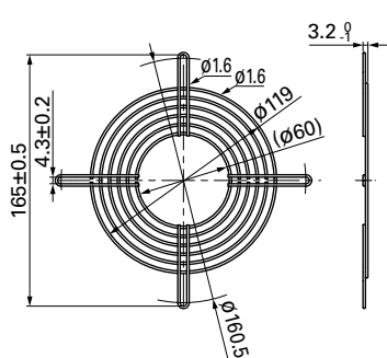
Outlet side
