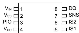
DS2751E 8-Pin TSSOP Package (Lead Free Available)
