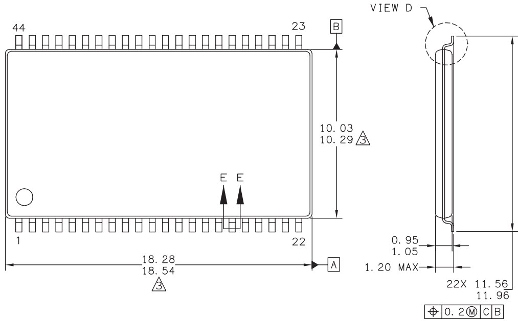
Figure 10 – 44-TSOP2 Package Outline
