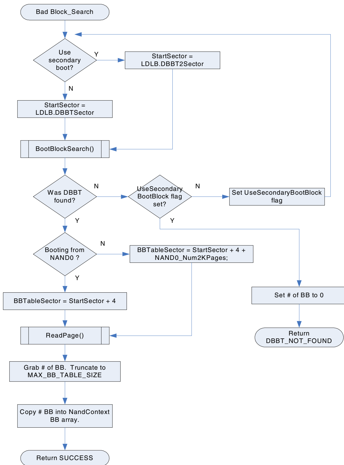
Figure 35-9. Bad Block Search
