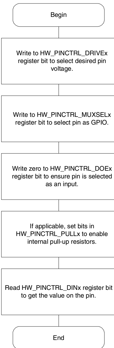
Figure 37-3. GPIO Input Setup Flowchart
