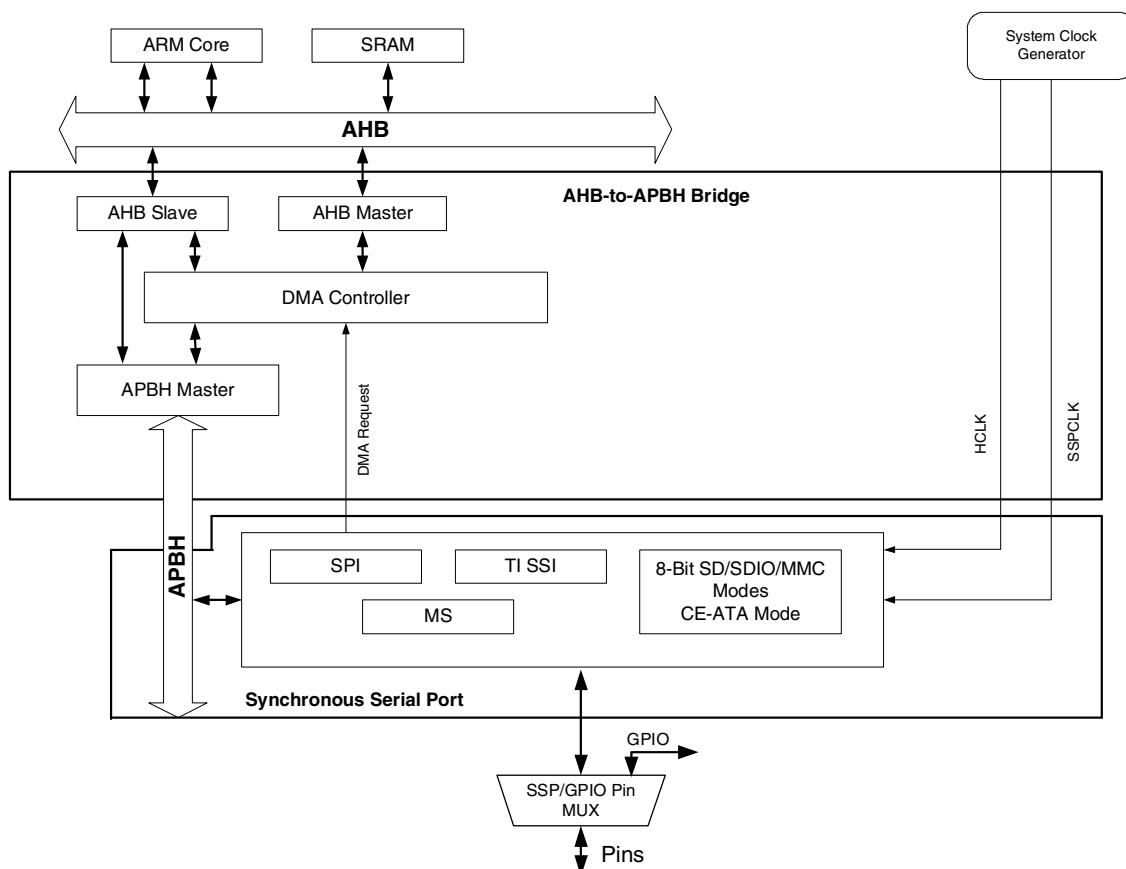
Figure 21-1. Synchronous Serial Port Block Diagram
