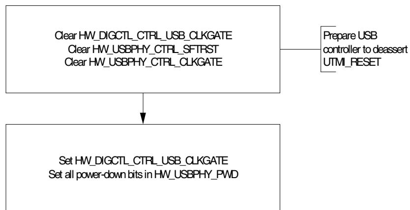
Figure 8-5. UTMI Powerdown
