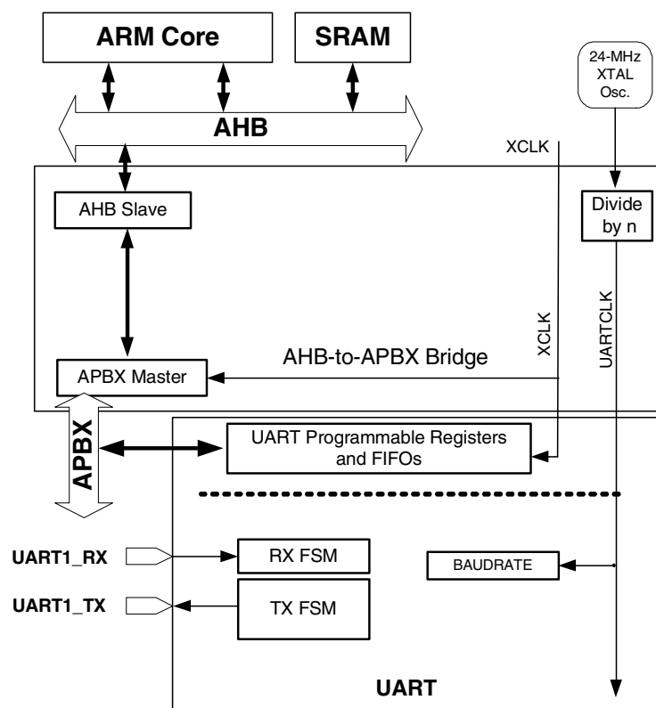
Figure 27-1. Debug UART Block Diagram
