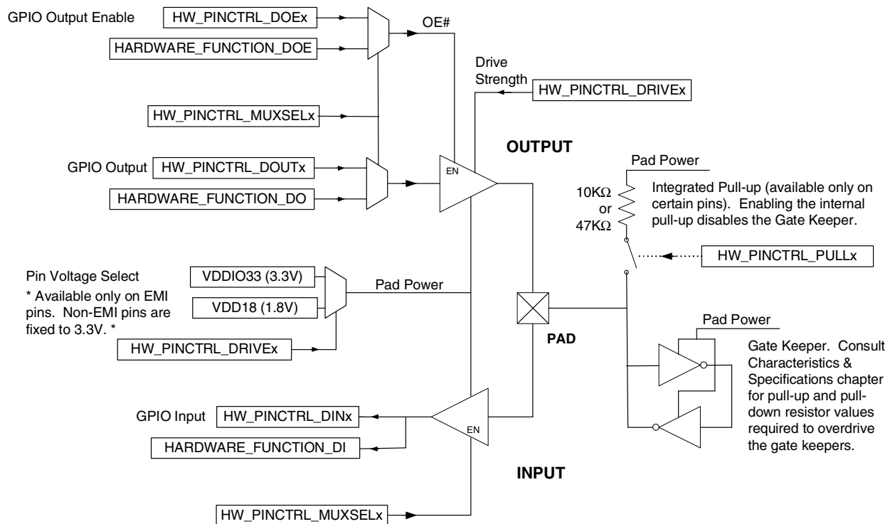
Figure 37-1. Pad Diagram
