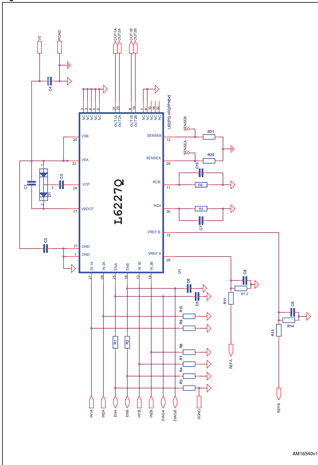
Figure 2. EVAL6227QR demonstration board schematic
