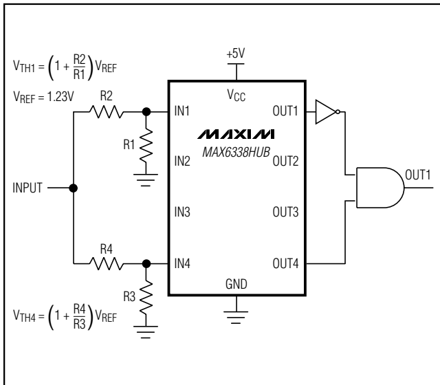
Figure 4. Window Detection
