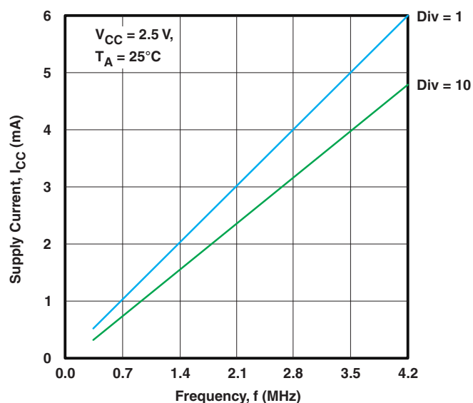
Figure 12. Supply Current vs Frequency ( V_{CC} = 2.5 V)
