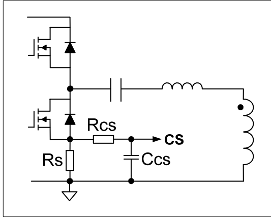
Figure 10: Current Sensing with a Sense Resistor
