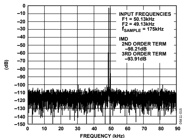
Figure 15. IMD Plot
