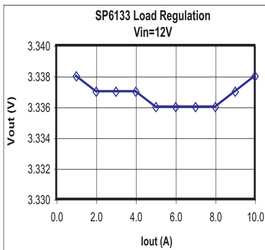
Figure 8: Load Regulation, 12V
