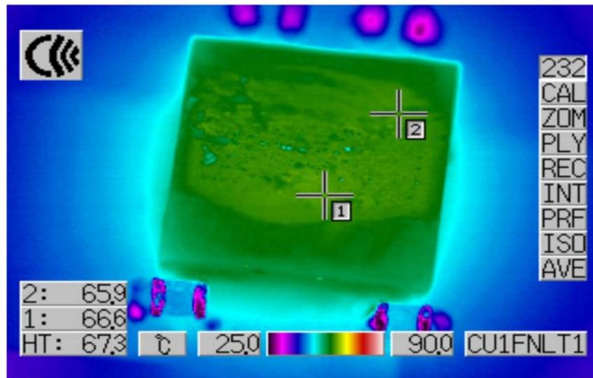
Figure 7. Thermal Capture at 5V_{IN} , 1.5V_{OUT} at 12A and 1.2V_{OUT} at 12A. Ambient Temperature = 30^{\circ}\text{C} , No Airflow and No Heat Sink
