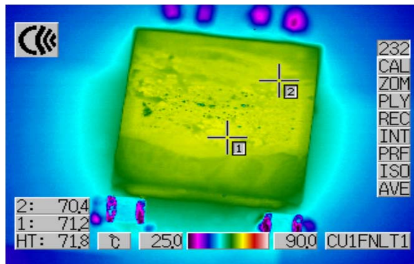
Figure 8. Thermal Capture at 5V_{IN} , 1.5V_{OUT} at 13A and 1.2V_{OUT} at 13A. Ambient Temperature = 30^{\circ}\text{C} , No Airflow and No Heat Sink
