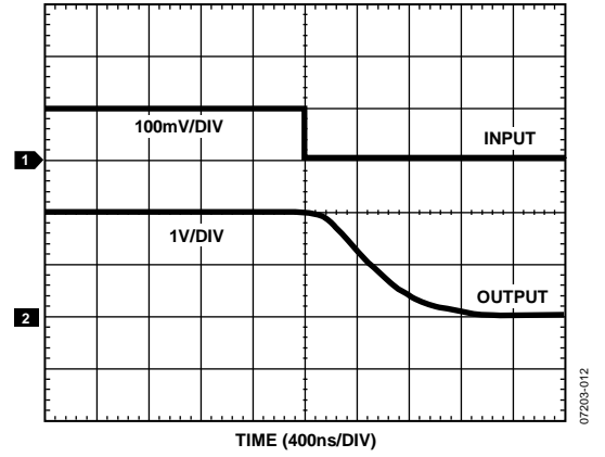
Figure 13. Fall Time
