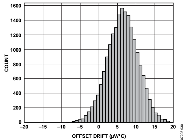
Figure 25. Offset Drift
