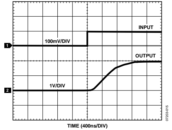
Figure 14. Rise Time
