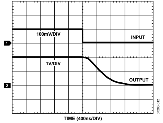
Figure 13. Fall Time
