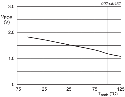
Fig 25. Power-on reset voltage versus temperature; falling V_{CC}
