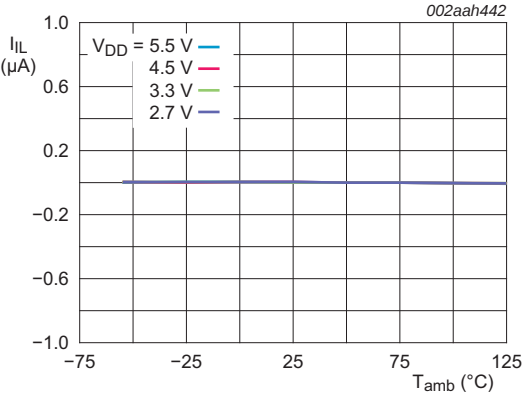
Fig 19. LOW-level input current versus temperature; digital pins
