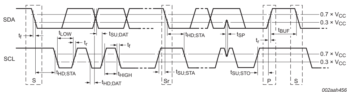
Fig 26. Timing diagram
