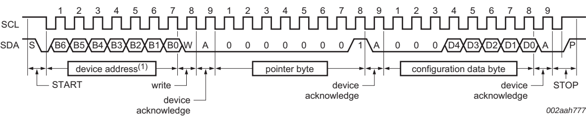
Fig 7. Write configuration register (1-byte data)
