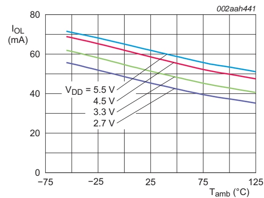
Fig 18. LOW-level output current on OS pin versus temperature; V_{OL} = 0.4\text{ V}
