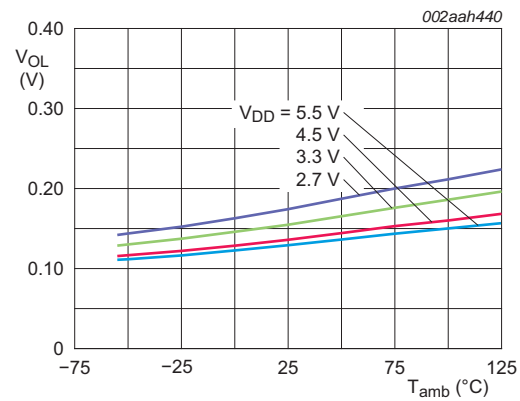
Fig 17. LOW-level output voltage on OS pin versus temperature; I_{OL} = 4\text{ mA}
