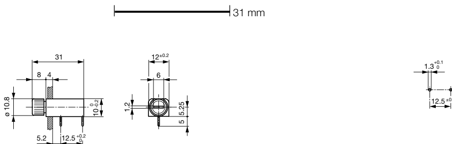
Drilling diagram
