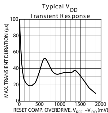
Figure 3b. Typical V_{DD} Transient Response
