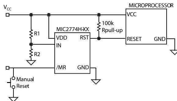
Figure 5. MIC2774H Valid RST Below 1.2V
