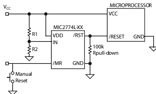
Figure 4. MIC2774L Valid /RST Below 1.2V
