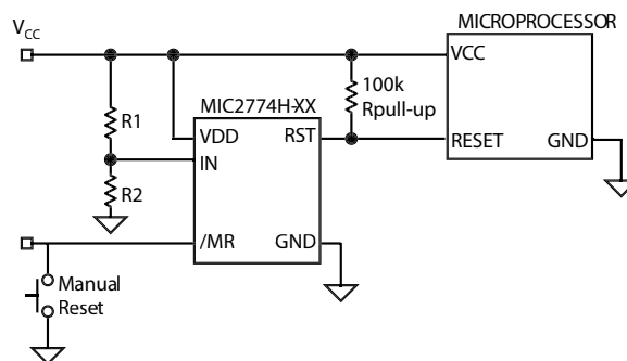
Figure 5. MIC2774H Valid RST Below 1.2V
