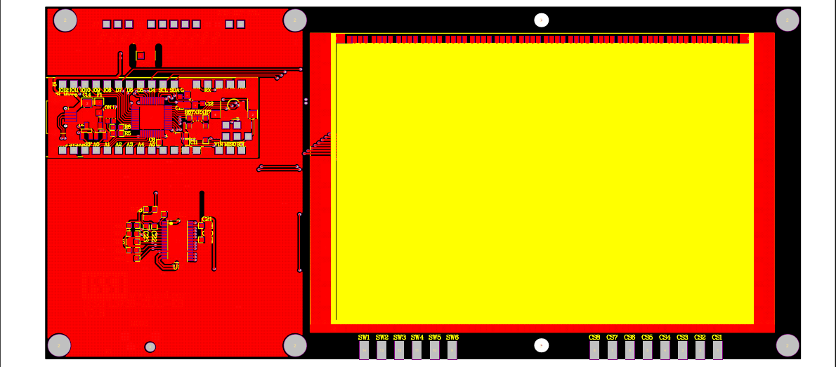
Figure 4: Board PCB Layout - Top Layer
