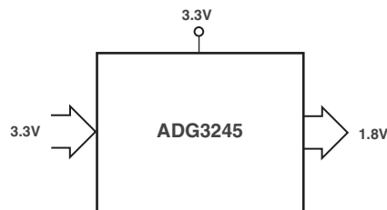
Figure 9. 3.3 V to 1.8 V Voltage Translation, \overline{SEL} = 0\text{ V}
