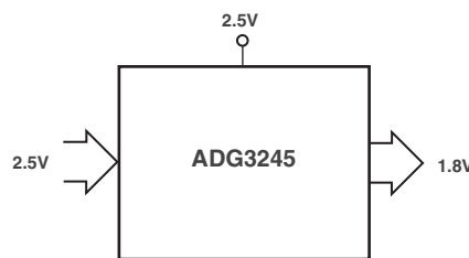
Figure 7. 2.5 V to 1.8 V Voltage Translation, \overline{SEL} = 2.5\text{ V}_{CC}
