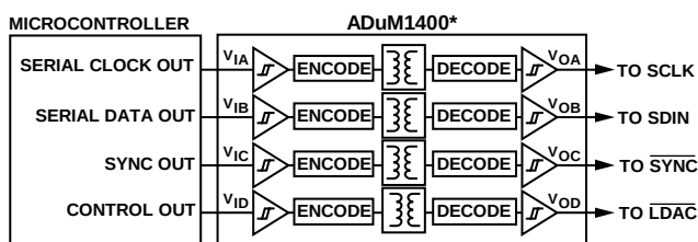
Figure 49. Isolated Interface
