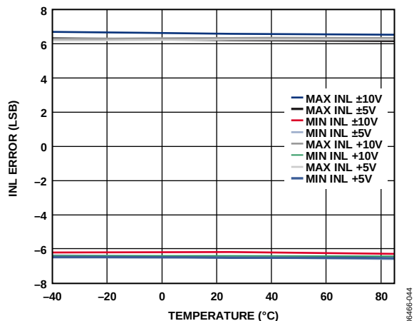
Figure 12. AD5752R Integral Nonlinearity Error vs. Temperature
