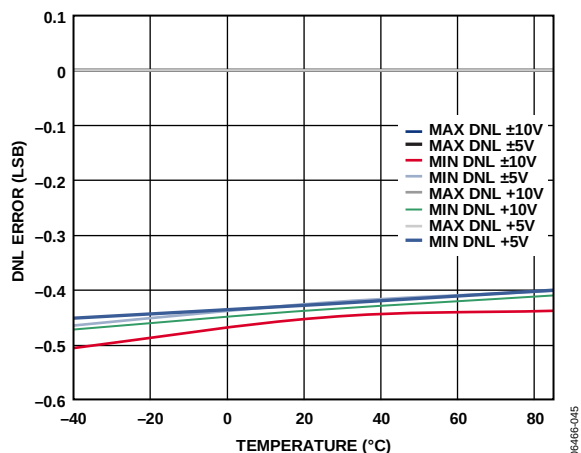
Figure 13. AD5752R Differential Nonlinearity Error vs. Temperature
