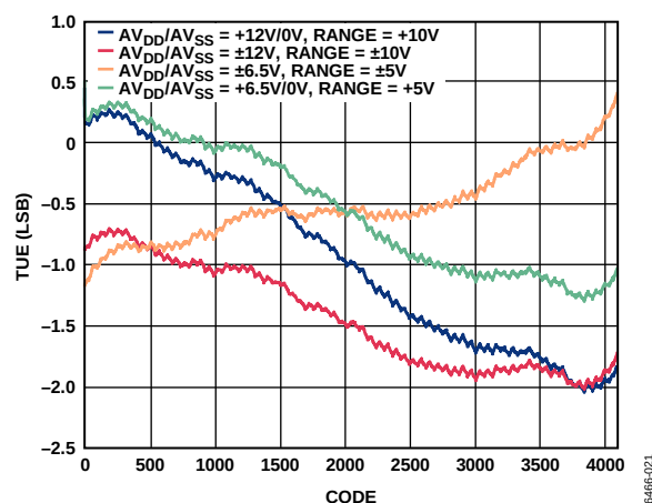
Figure 39. AD5722R Total Unadjusted Error vs. Code
