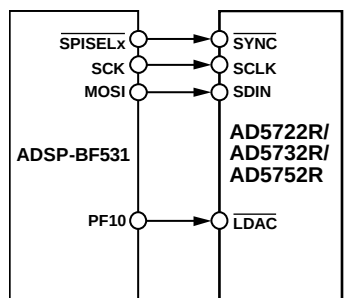
Figure 50. AD5722R/AD5732R/AD5752R-to-Blackfin Interface
