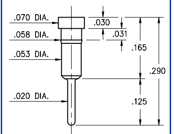
1942-0-00-XX-00-00-03-0 Press-fit in .057 mounting hole
