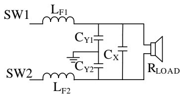
Figure 5: BTL Filter Configuration
