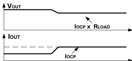
Figure 23. Overload
