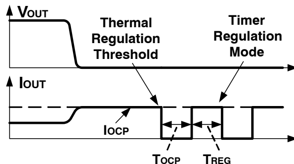
Figure 24. Short circuit
