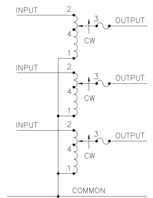
SCHMATIC FUSE RECOMMENDED BUT NOT SUPPLIED
