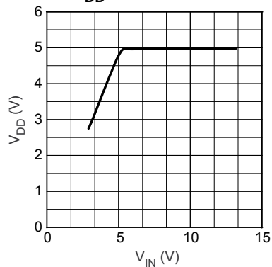
V_{DD} Line Regulation
