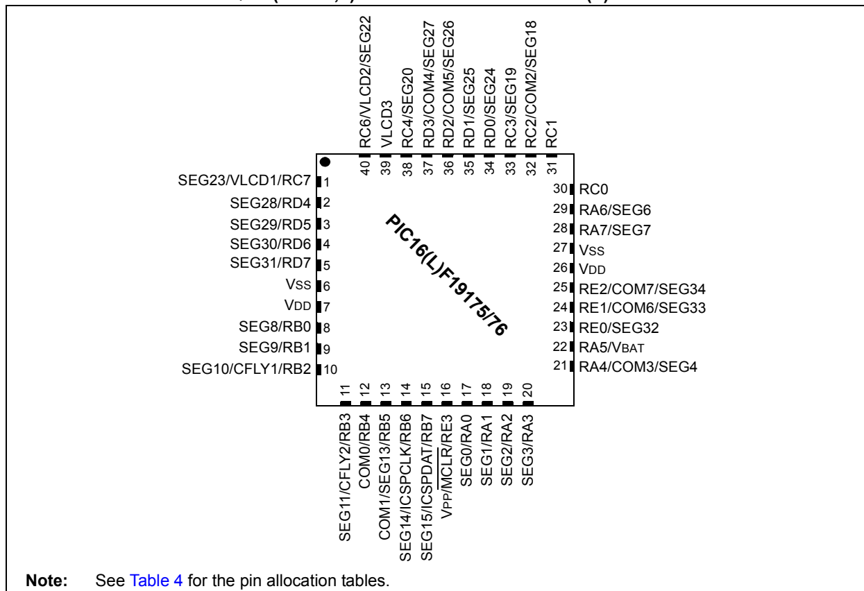
FIGURE 4: 40-PIN UQFN (5X5X0,5) PIN DIAGRAM FOR PIC16(L)F19175/76
