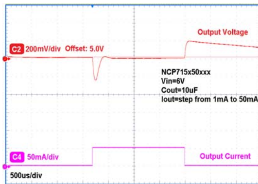
Figure 36. Load Transient Response
