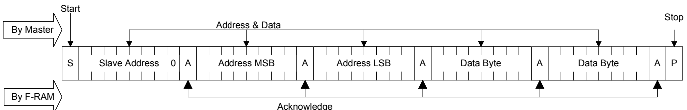
Figure 9. Multi-Byte Write
