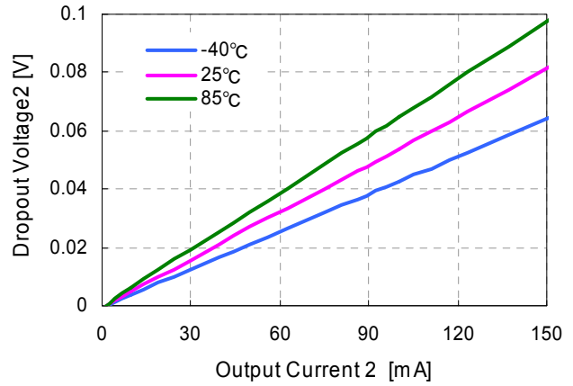
RP600K2xxC LDO=3.3V
