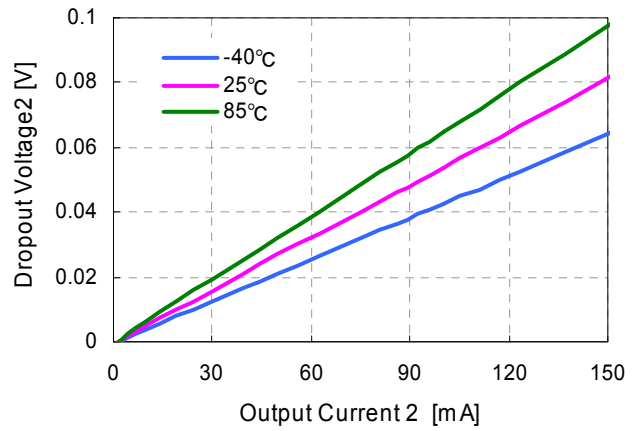
RP600K2xxC LDO=3.3V
