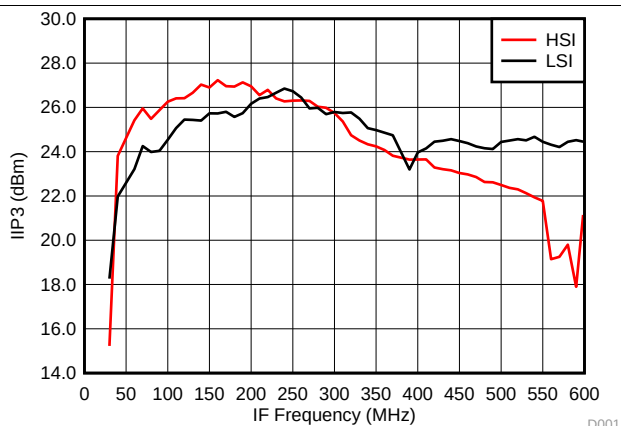
Figure 8. IIP3 vs IF Frequency over H/LSI
