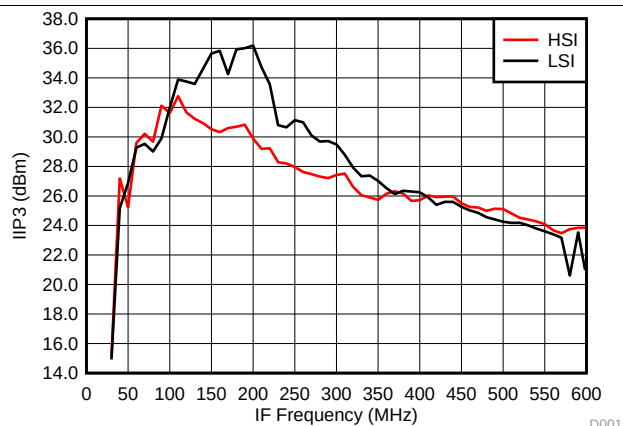
Figure 32. IIP3 vs IF Frequency over H/LSI
