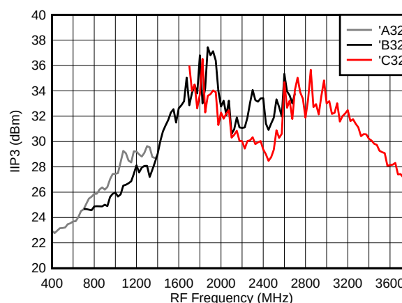
IIP3 Performance Across Frequency
