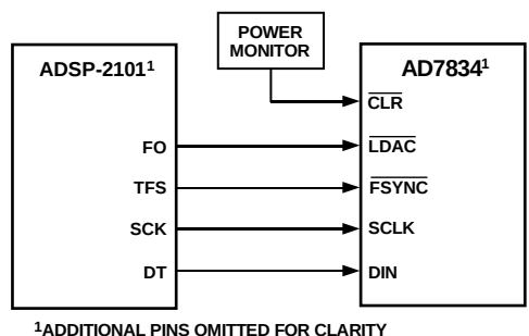
Figure 28. AD7834 to ADSP-2101 Interface
