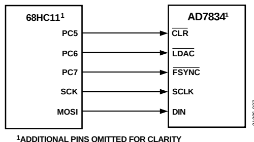
Figure 27. AD7834 to 68HC11 Interface
