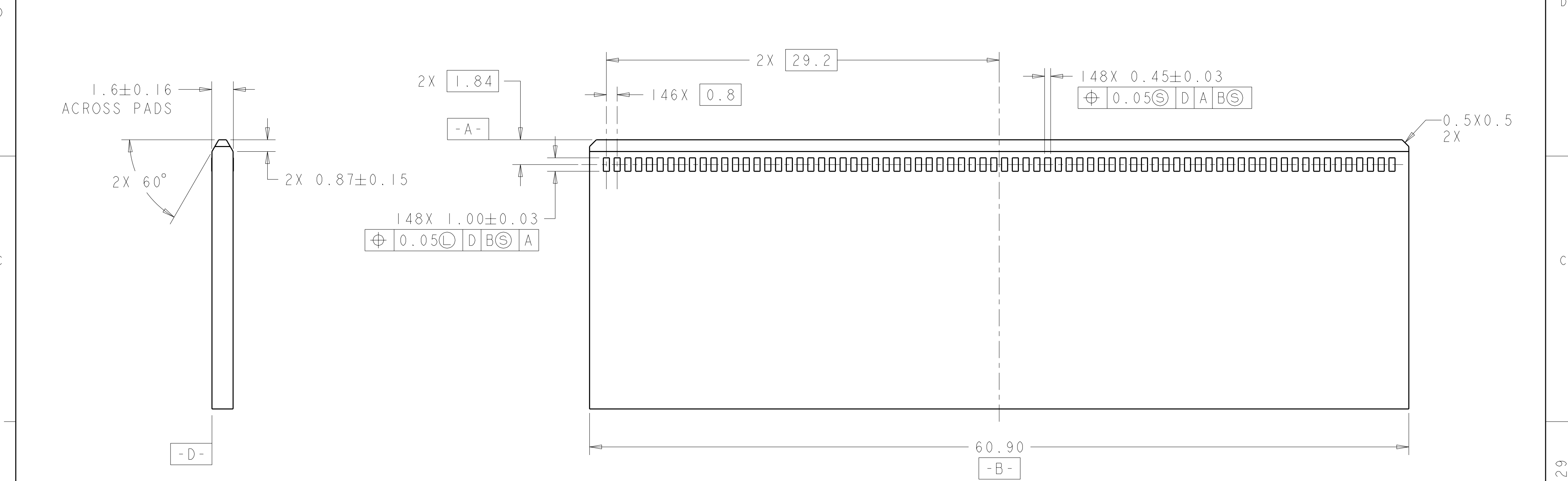
REQUIRED MODULE PC BOARD DIMENSIONS
