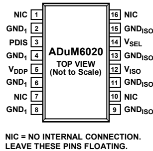
Figure 5. Pin Configuration
