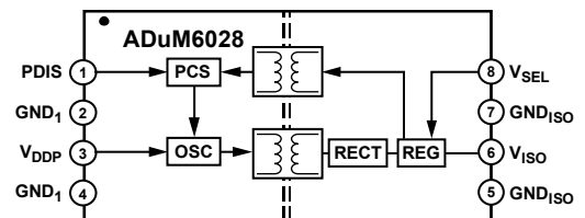
Figure 2. ADuM6028 Functional Block Diagram
