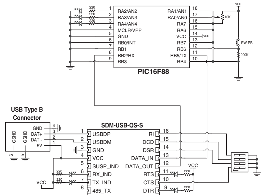
Figure 14: Interface with a Microprocessor
